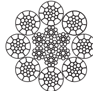
Dyform 8
