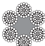
6x47 Warrington - Seale 1+6/8+(8+8)+16
