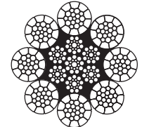
Dyform Bristar 8
