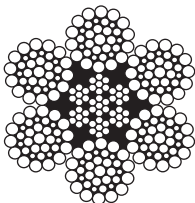
6x36 Warrington - Seale 1+7+(7+7)+14
