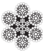
6x41 Warrington-Seale 1+8+(8+8)+16
