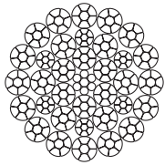
Dyform 34LR
