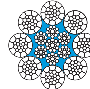
Dyform 8 PI
