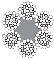
6x36 Warrington - Seale 1+7+(7+7)+14
