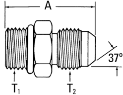
SAE O-Ring boss/37° flare (continued)
