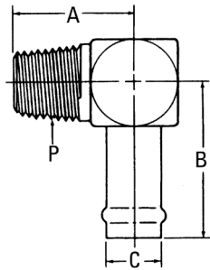
Part no. FF1162-(Dash size) (Ref. SAE 430260)
