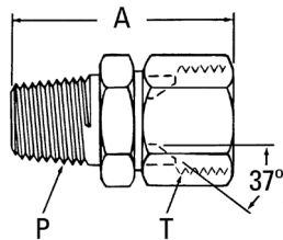
Part no. 2018-(Dash size)
