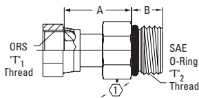
Part no. FF2130T-(Dash size) (Ref. SAE 520181)
