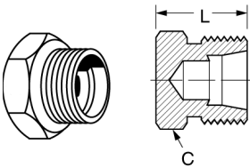
Part no. 7229x (Ref. SAE No. 080109)
